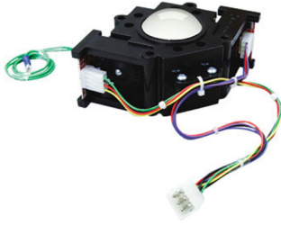
Happ Trackball
